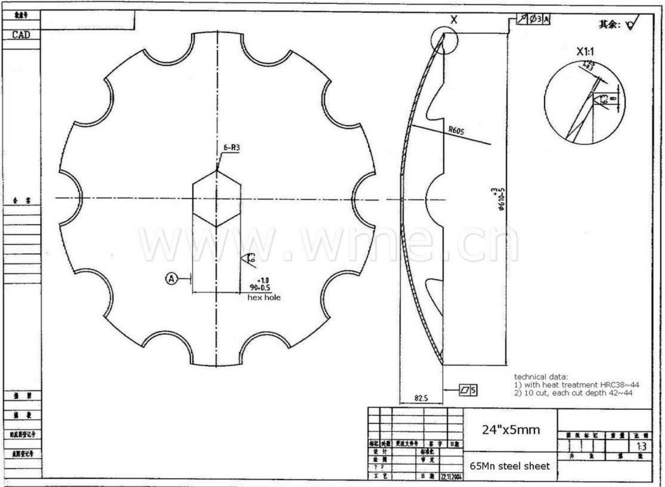
harrow disc 24"x5mm cut type with hex hole
