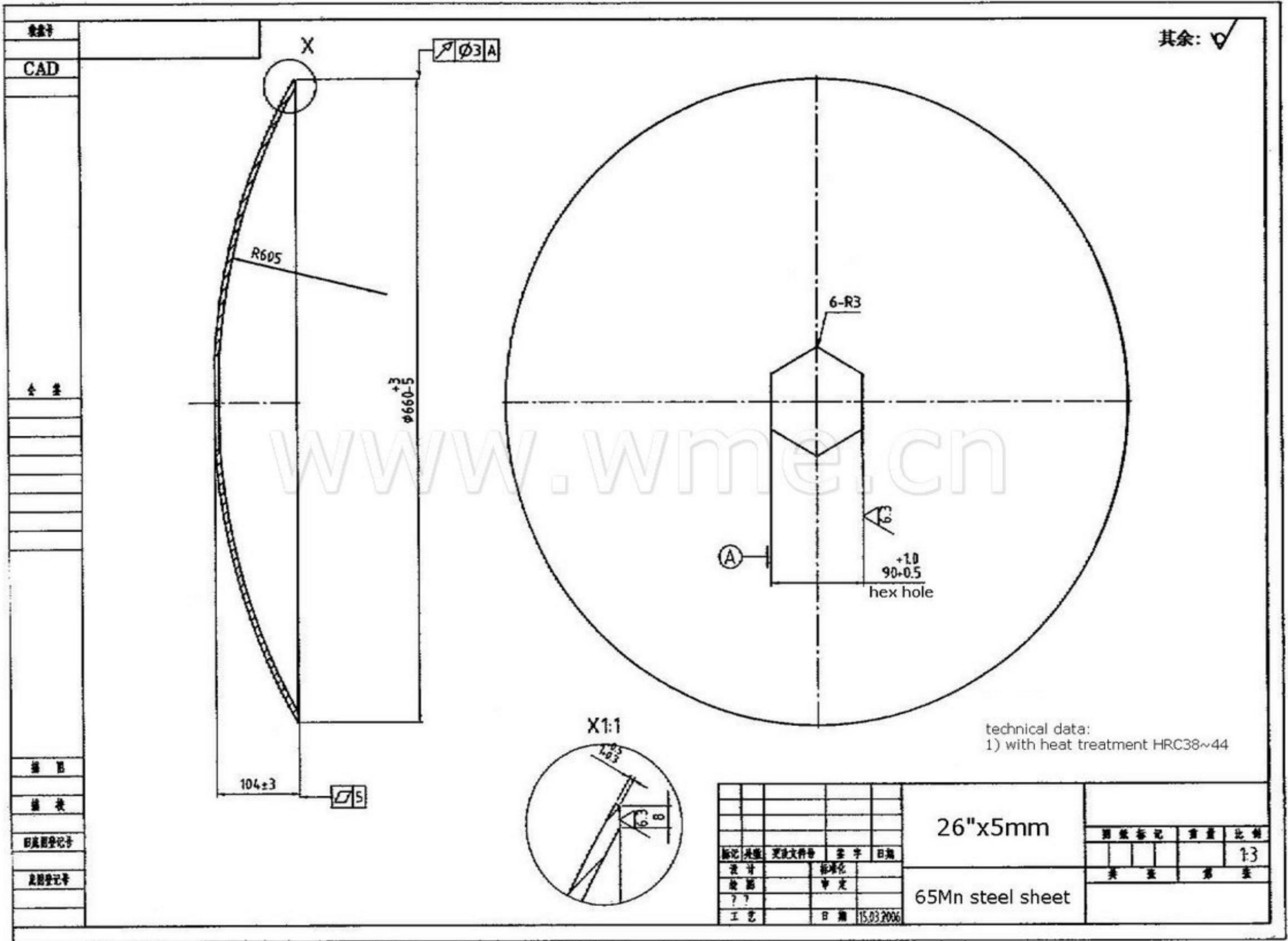
harrow disc 26"x5mm plain type with hex hole
