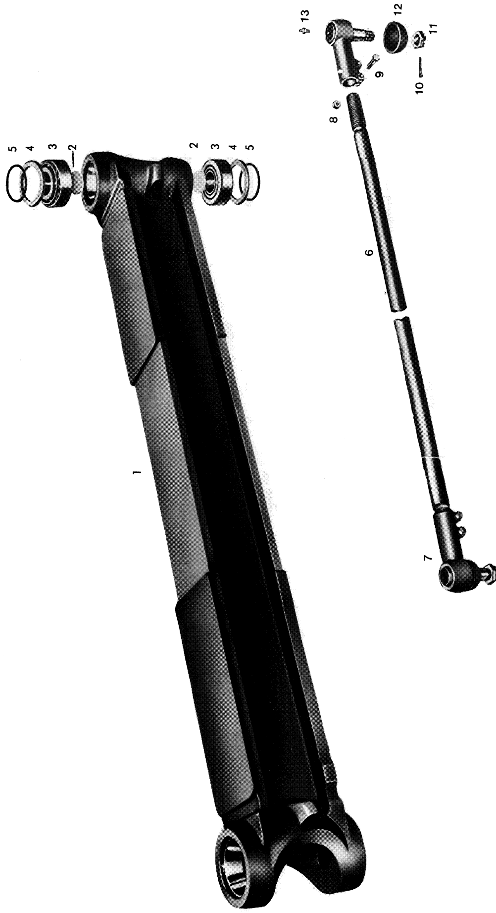
Tafel/Table 4 Achsbrücke, Spurstange Axle housing, Tie rod
