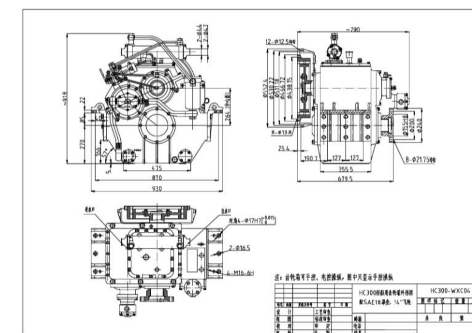
SAE1#罩壳 14"齿形块-WXC04
