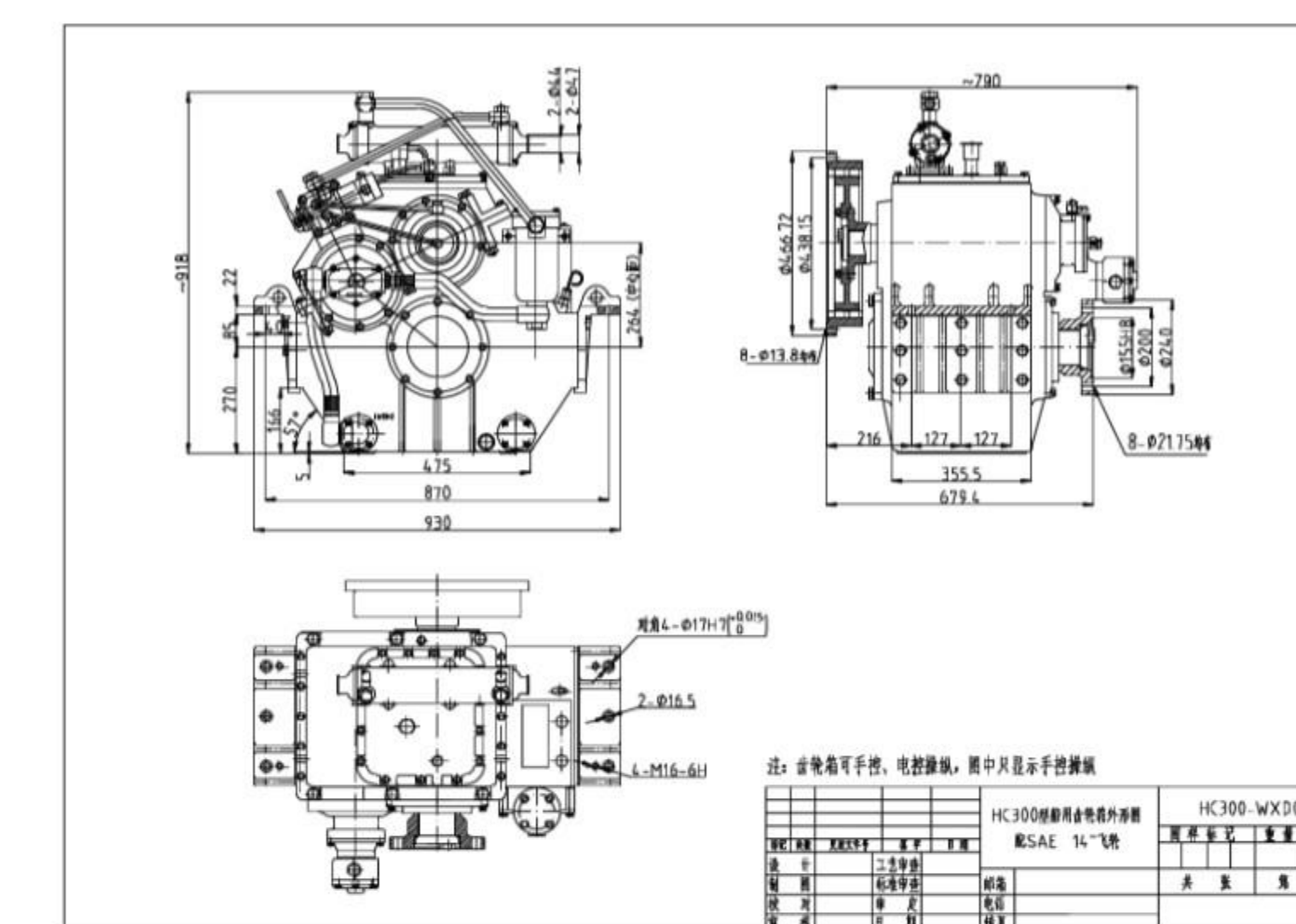
SAE14"齿形块-WXD03
