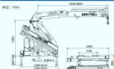
SQ5ZK3Q 起重能力曲线图 CURVE GRAPH OF LIFTING CAPACITY
