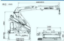
SQ5ZK2Q 起重能力曲线图 CURVE GRAPH OF LIFTING CAPACITY
