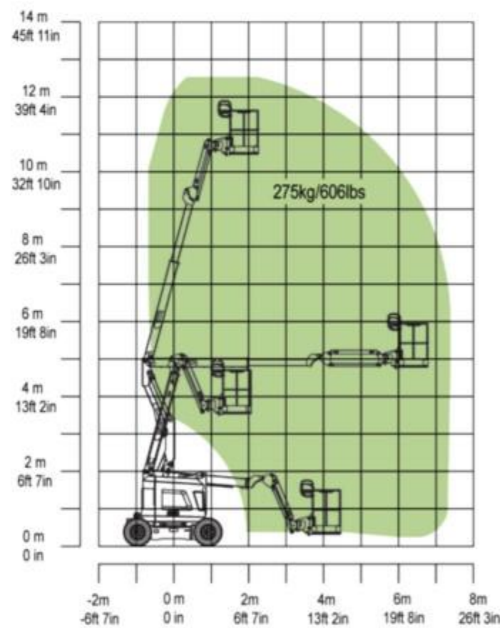
Range of Jib Swing Motion ZA10J
