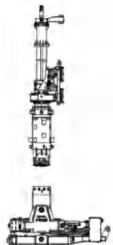
3.Cased Kelly drilling with oscillator 护筒跟进配搓管机
