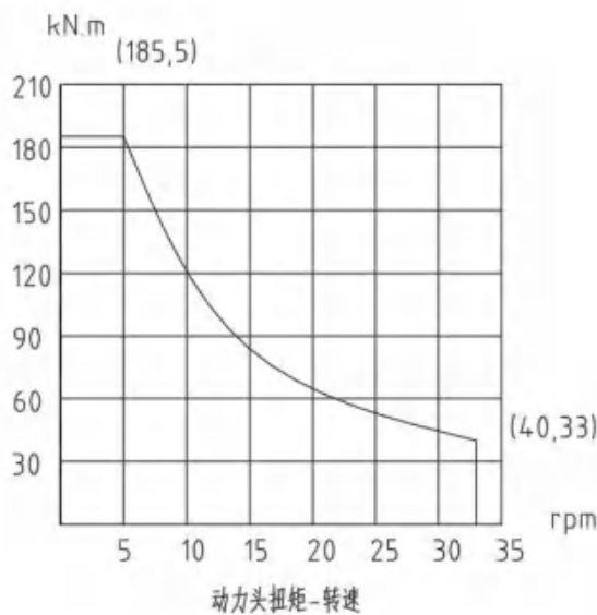
Rotary Drive-Torque Diagram
